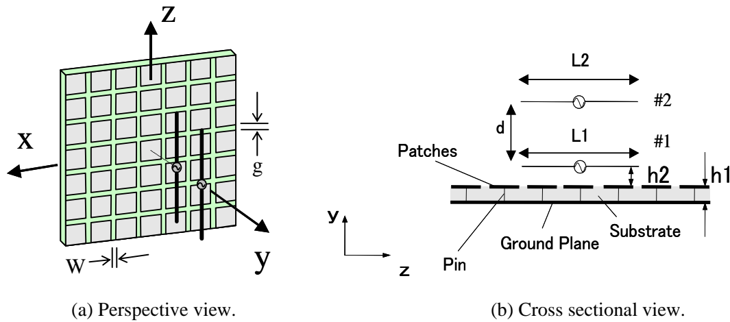
Fig. 1. Structure of two element phased array dipole antenna on EBG substrate.
