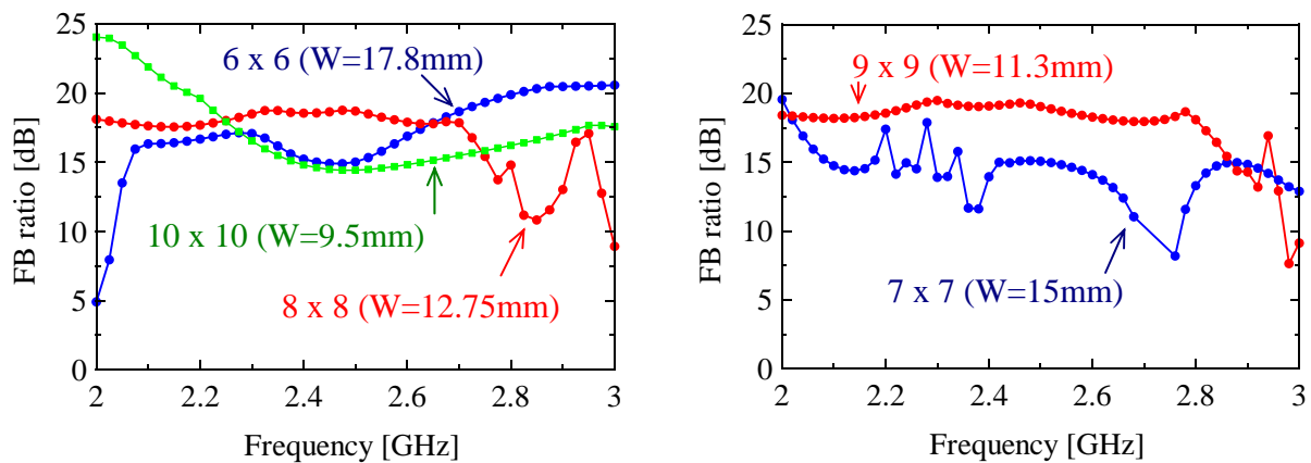
Fig. 2. Front-to-back ratio for different number of EBG patches, g = 3 mm.
